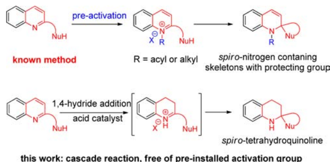
Scheme 1. Proposed Synthesis of Spiro -tetrahydroquinolines from Quinolines
