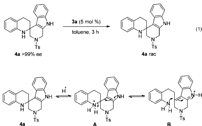
Scheme 3. Epimerization of 4a under Acidic Conditions
